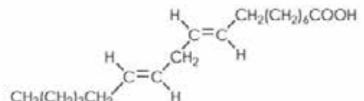
trans,trans -9,12-oktadekadienska kiselina
