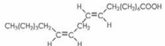
cis,trans -9,12-oktadekadienska kiselina
